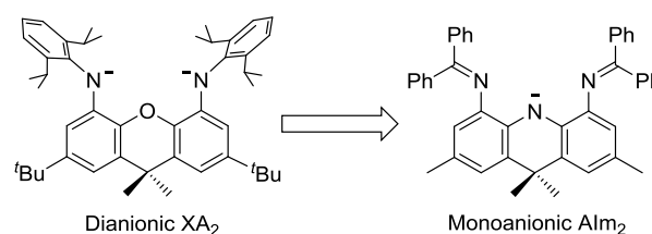
Figure 1. Relationship between the XA 2 and Alm 2 ligands.
