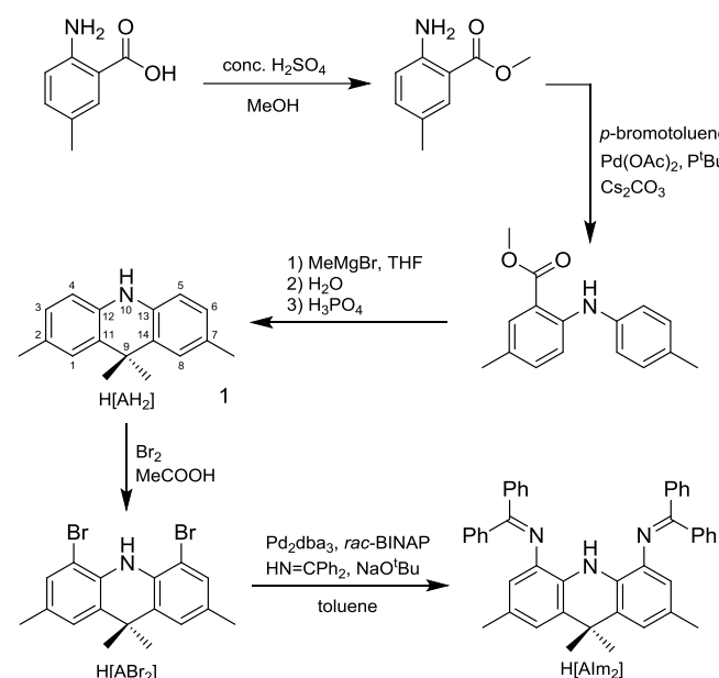
Scheme 1. Synthetic route to the H[Alm 2 ] proligand.
