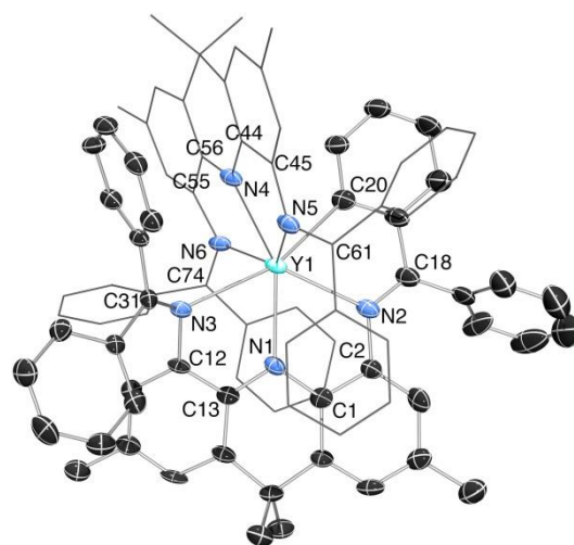
Figure 4. Single crystal X-ray structure of 1 \cdot (\text{pentane})_{0.5}(\text{toluene})_2 . Hydrogen atoms and lattice solvent have been removed. Except for nitrogen atoms, the unactivated \text{Alm}_2 ligand is depicted in wireframe for clarity. Thermal ellipsoids are set at 50% probability. Selected bond lengths [Å]: Y1–N1 2.367(4), Y1–N2 2.529(4), Y1–N3 2.662(4), Y1–N4 2.358(4), Y1–N5 2.494(4), Y1–N6 2.475(5), Y1–C20 2.466(5), N1–C1 1.391(7), N1–C13 1.374(6), N2–C2 1.438(6), N2–C18 1.303(7), N3–C12 1.445(6), N3–C31 1.303(6), N4–C44 1.374(7), N4–C56 1.385(7), N5–C45 1.423(7), N5–C61 1.305(7), N6–C55 1.417(6), N6–C74 1.317(6).
