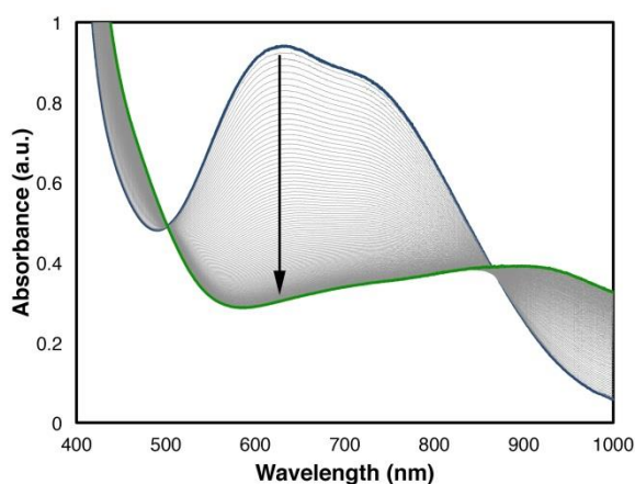
Figure 9. Absorption spectra for the conversion of 1 to 2 recorded from 0.5 to 60 h in benzene.
