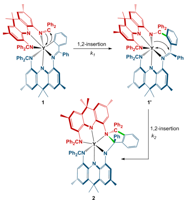
Scheme 3. Proposed reaction pathway for conversion of 1 to 2 .
