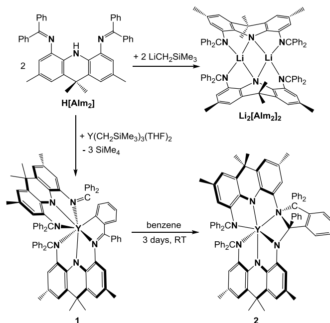
Scheme 2. Synthesis of 1 , 2 and \text{Li}_2[\text{Alm}_2]_2 . In the structure of 2 , an interaction between yttrium and an ortho carbon atom of one of the isoindoline phenyl rings is not shown.
