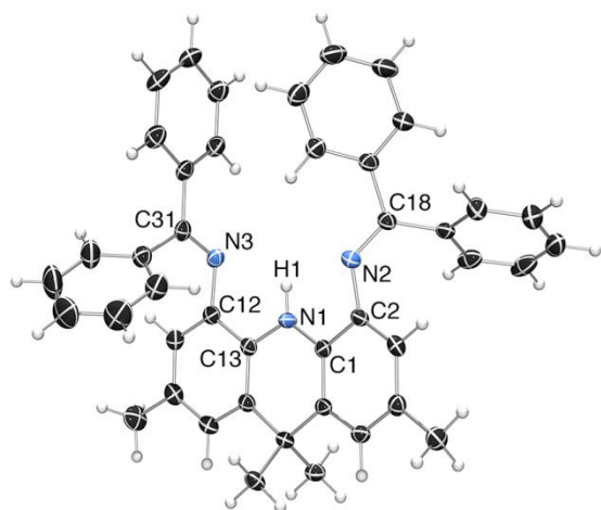
Figure 3. Single crystal X-ray structure of \text{H}[\text{Alm}_2] . Thermal ellipsoids are set at 50% probability. Selected bond lengths [Å]: N1–C1 1.3782(17), N1–C13 1.3828(17), N2–C2 1.4155(16), N2–C18 1.2833(16), N3–C12 1.4250(16), N3–C31 1.2839(17).
