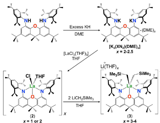
Scheme 2 Synthesis of [\text{K}_2(\text{XN}_2)(\text{DME})_x] and Complexes 2 and 3 .
