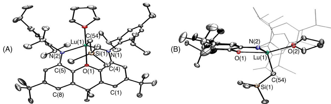
Fig. 2 Two views of the X-ray crystal structure for 1 \cdot (\text{C}_6\text{H}_6)_{0.5} . Ellipsoids are set to 50 %. Hydrogen atoms and lattice solvent are omitted. The tert -butyl groups are rotationally disordered over two positions, and only one is shown for clarity. In view B the 2,4,6-trisopropylphenyl groups are depicted in wire-frame format. Selected bond lengths [Å] and angles [°]: Lu–N(1) 2.221(2), Lu–N(2) 2.228(2), Lu–C(54) 2.326(2), Lu–O(1) 2.299(1), Lu–O(2) 2.264(1), N(1)–Lu–N(2) 130.41(6), N(1)–Lu–C(54) 106.09(7), N(2)–Lu–C(54) 110.41(7), O(1)–Lu–C(54) 104.38(6), O(2)–Lu–C(54) 97.56(7), O(2)–Lu–N(2) 105.39(6), O(2)–Lu–N(1) 101.76(6).
