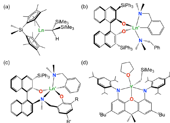
Fig. 1 Highly Active Rare Earth Catalysts for Intermolecular Hydroamination of Unactivated Alkenes (Ln = Nd; Ln' = Y).
